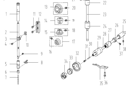
3. 针杆、竖轴、下轴部件/Needle bar & Upright Shaft & Hook Driving Shaft Compon
