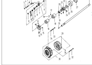
2. 上抽轴组件分件/Main Shaft & Thread Take-up Components
